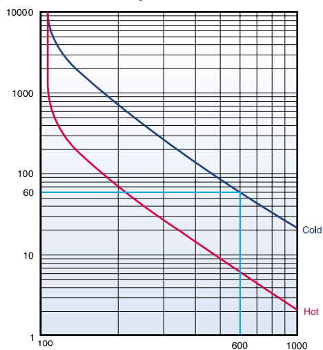
Trip class 60
