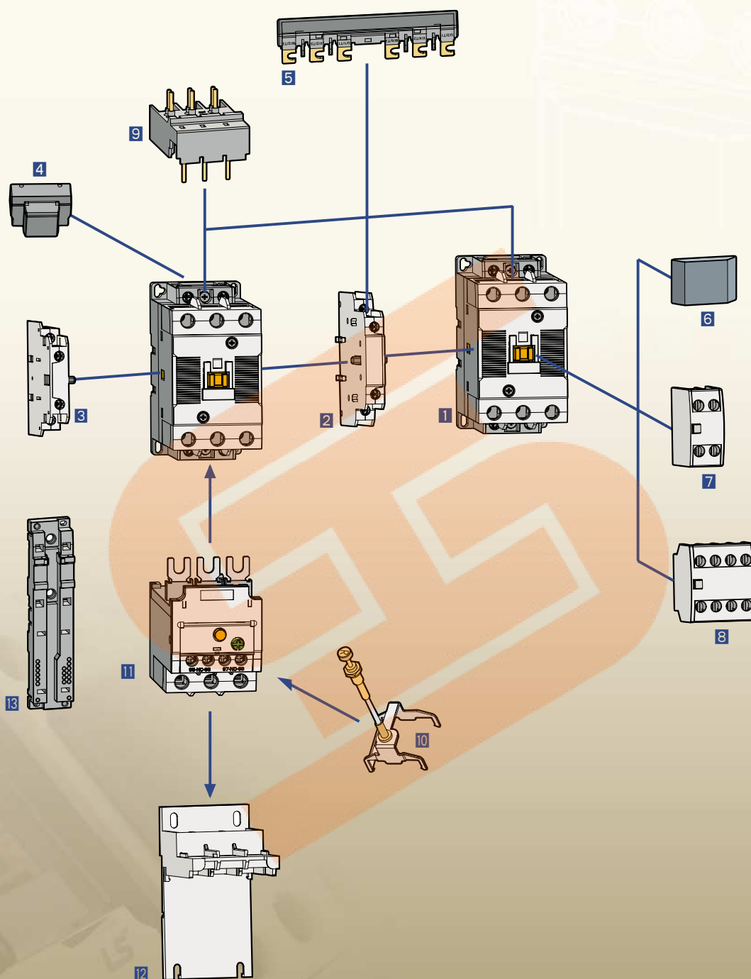
Accessory layout upto 150AF
