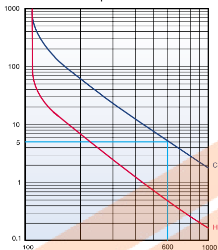
Trip class 5
