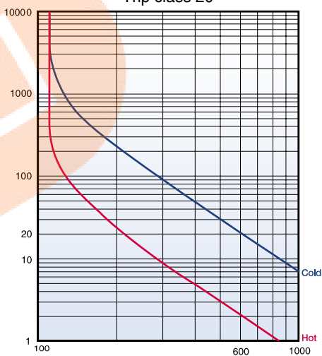
Trip class 20
