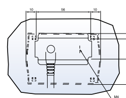
Panel cutting size
