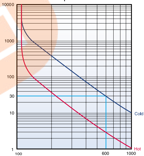
Trip class 30
