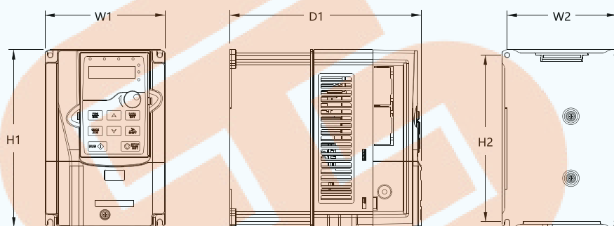
380V 1.5-37kW VFD wall mounting diagram
