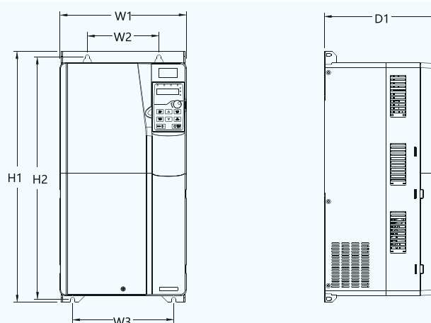
380V 45-75kW VFD wall mounting diagram
