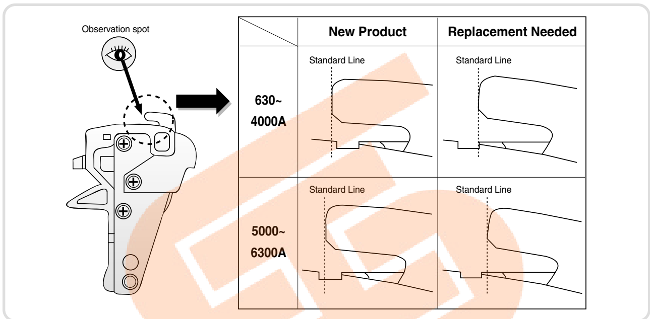
Fig 8. The standard figure for contact replacement
