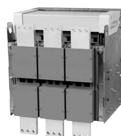
Fig.6 Front type
