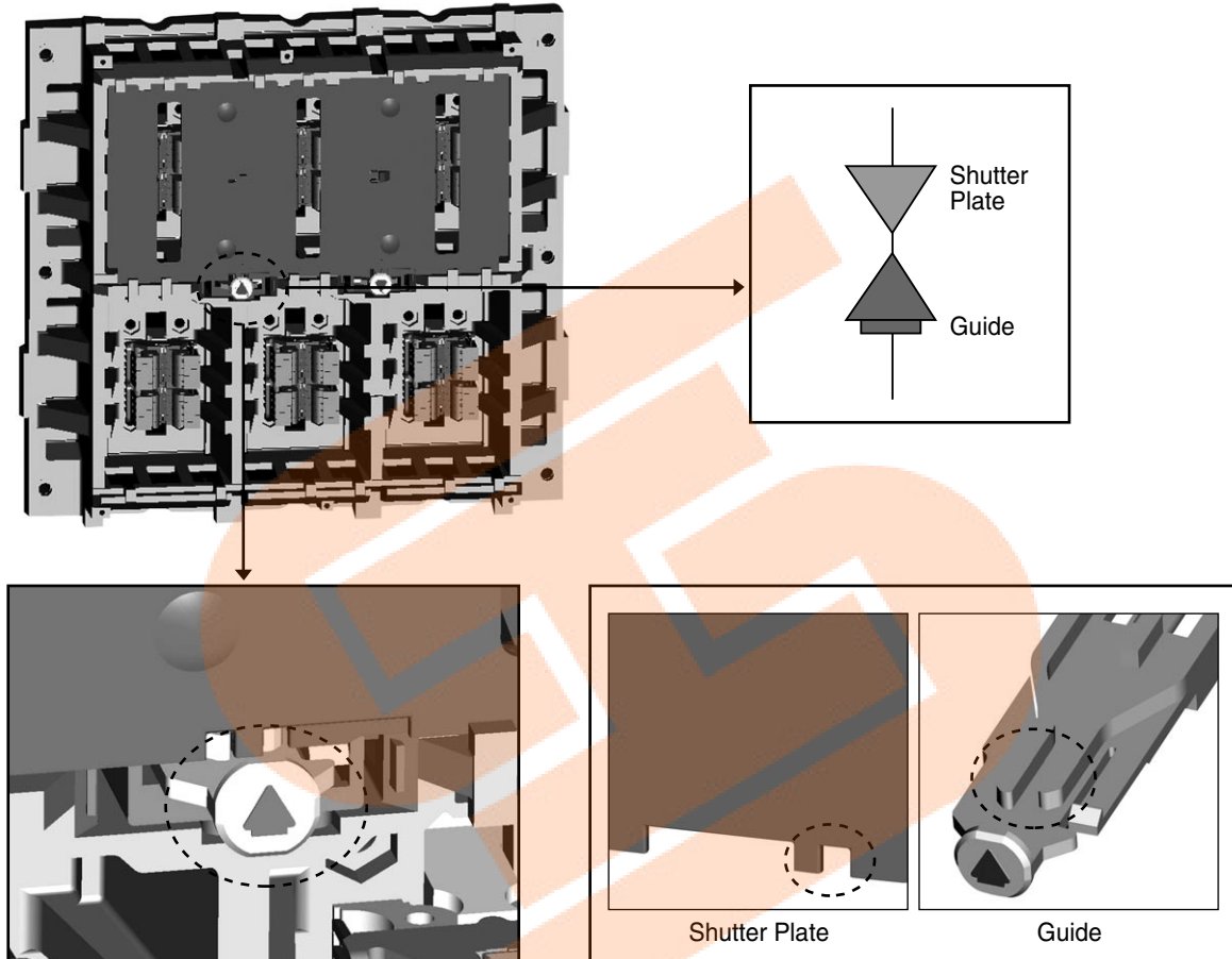
Projections and groove for operating Shutter plate
