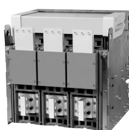
Fig.5 Front/Vertical type
