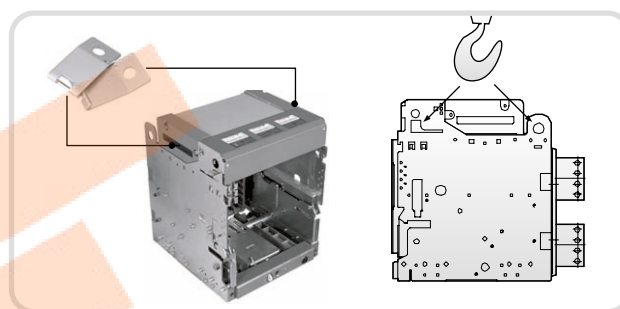
Fig. 3. Transporting method of Draw-out type
